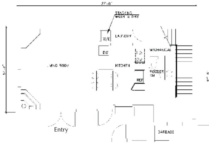
First Floor 768 sq ft.
